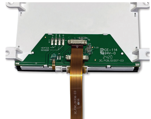
Replacement LCD front and back 76-50248-00
